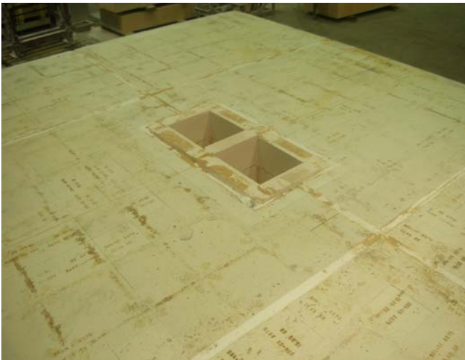
16' x 18' kiln car for 1610°C – after 1 year service
